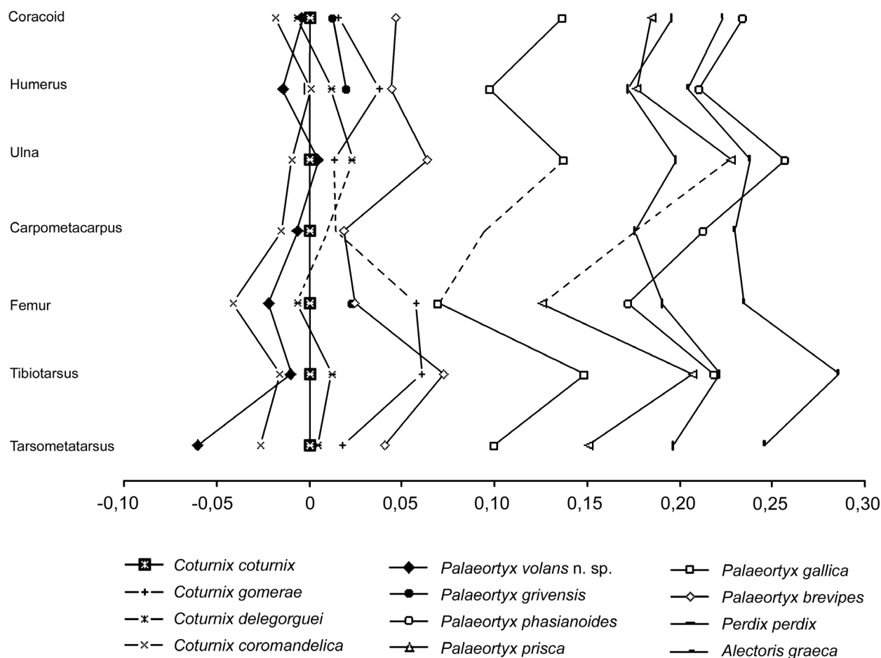
Figure 3 - Ratio diagram of the log differences of the mean dimensions of the long bones of Palaeortyx volans n. sp. compared with those of Coturnix coturnix (selected as standard), C. gomeræ , C. delegorguei , C. coromandelica , Palaeortyx grivensis , P. phasianoides , P. prisca , P. gallica , P. brevipes , Perdix perdix and Alectoris graeca (data from Kraft, 1974; Jaume et al., 1993; Göhlich & Mourer-Chauviré, 2005)
